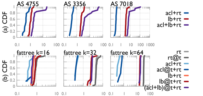
Figure 4: CDF of orchestration delay: normalized per-rule orchestration delay (ms) on various network sizes.
